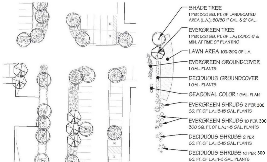
Figure 3-2 – Parking Lot Design
